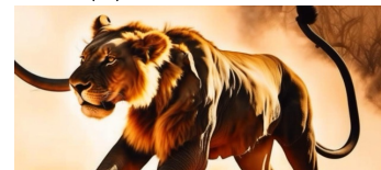
(f) Attn-SF
