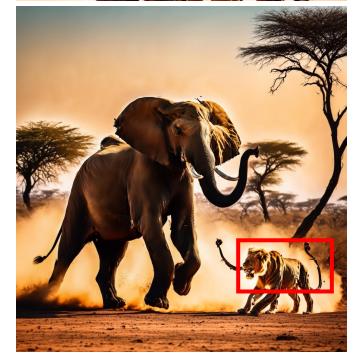
(i) +DIC
