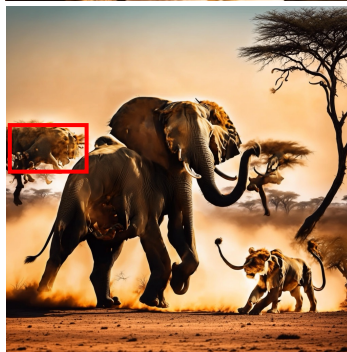
(h) PG
